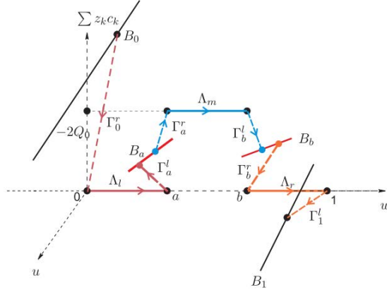
Figure 1: An illustration of a singular connecting orbit projected to the space of (u, z_1 c_1 + z_2 c_2, w) . Boundary layers at w = 0 and w = 1 exist if electroneutrality boundary conditions are not assumed.
