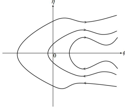
Figure 1: Sketch of the phase plane portrait for Case I: \gamma_1 > |\gamma_2| .
