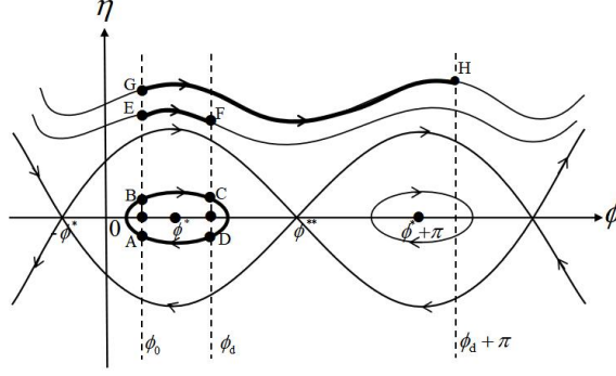
Figure 8: Types of solutions in Case III1 with -\gamma_2 > \gamma_1 > 0 and \int_0^\pi \frac{h(t)}{g(t)} dt = 0 : monotone 0-winding solutions represented by the arc EF from E to F and the arc BC, monotone 1-winding solution represented by the arc GH; the arc ABC represents a non-monotone ( l -1-vibrating) solution, the arc BCD represents a non-monotone ( r -1-vibrating) solution, the arc ABCD represents a ( l, r )-2-vibrating solution, etc.
