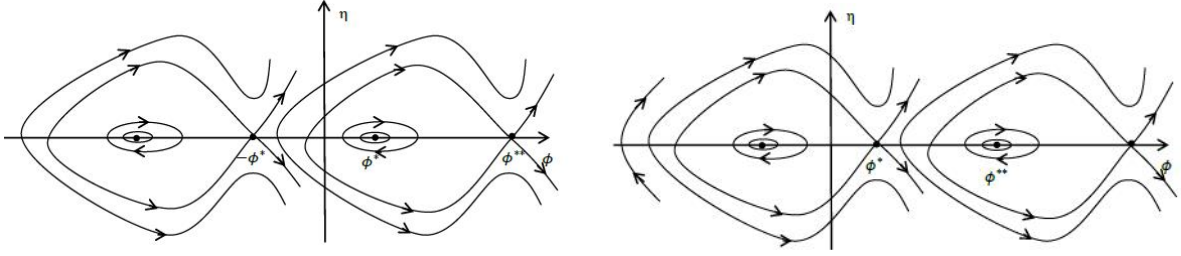
Figure 5: Phase plane portrait for Case III2 with \int_0^\pi \frac{h(t)}{g(t)} dt > 0 . Left panel: -\gamma_2 > \gamma_1 > 0 . Right panel: \gamma_2 > \gamma_1 > 0 .
