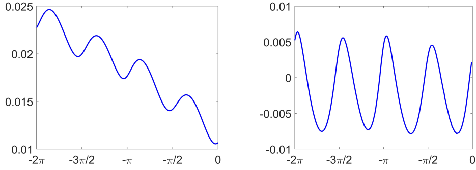
Figure 11: The graphs of N_m(\alpha) and N'_m(\alpha) : left for N_m(\alpha) and right for N'_m(\alpha) .
