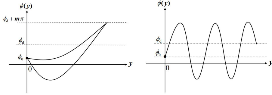
Figure 10: The graphs of \phi(y) . Left: top graph corresponds to a monotone m -winding solution and the bottom one is a non-monotone m -winding solution; Right: a (r, r) -5-vibrating solution.
