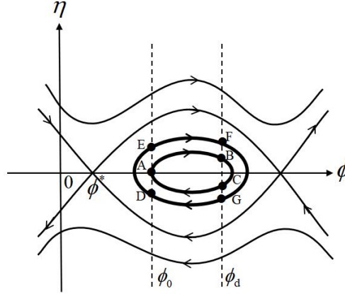
Figure 14: Representative orbits from Theorem 6.6: arc ABC represents the r -1-vibrating solution associated to a = \hat{a}_1 , arc EFG represents an r -1-vibrating solution for a > \hat{a}_1 , arc DEFG represents a (l, r) -2-vibrating solution associated to a > \hat{a}_1 ; arc ABCAC represents the (r, l) -2-vibrating solution for a = \hat{a}_2 , arc EFGDEFG represents an (r, l) -2-vibrating solution for a > \hat{a}_2 , arc DEFGDEF represents a (l, l) -3-vibrating solution for a > \hat{a}_2 .
