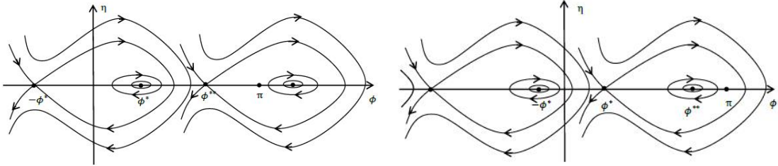
Figure 4: Phase plane portrait for Case III2 with \int_0^\pi \frac{h(t)}{g(t)} dt < 0 . Left panel: -\gamma_2 > \gamma_1 > 0 ; Right panel: \gamma_2 > \gamma_1 > 0 .
