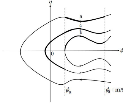
Figure 6: Three types of solutions in Case I for m \geq 0 : arcs a and b represent two monotone solutions and arc c represents a non-monotone solution.
