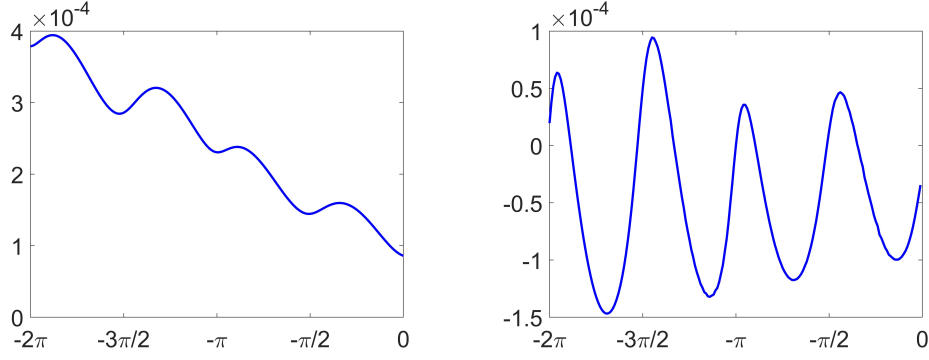
Figure 12: An example of graphs of L_m(\alpha) and L'_m(\alpha) : left for L_m(\alpha) and right for L'_m(\alpha) .
