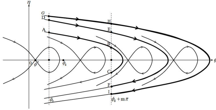
Figure 15: Representative orbits of non-monotone m -winding solutions from Theorem 6.7: arcs ABC , DEF , GHI in different regions separated by homoclinic orbits.
