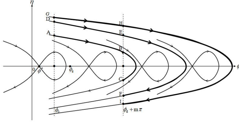
Figure 9: For Case III2 with \gamma_2 > \gamma_1 > 0 and \int_0^\pi \frac{h(t)}{g(t)} dt < 0 (homoclinic orbits to the right-hand side of saddles (\phi^* + n\pi, 0) ): in addition to possible solutions within the first homoclinic orbits as those in Case III1 above, the arcs AB, DE, GH represent three monotone m -winding solutions; the arcs ABC, DEF, GHI represent three non-monotone m -winding solutions.
