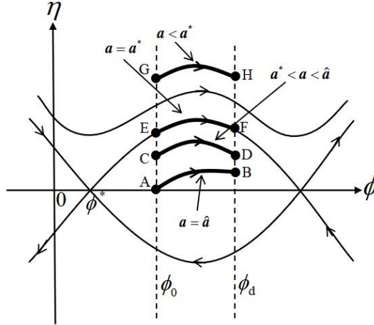
Figure 13: Representative orbits from Theorem 6.3 for \gamma_2 > 0 : arc AB associated to a = \hat{a} , arc CD associated to a \in (a^*, \hat{a}) , arc EF associated to a = a^* , and arc GH associated to a < a^* .
