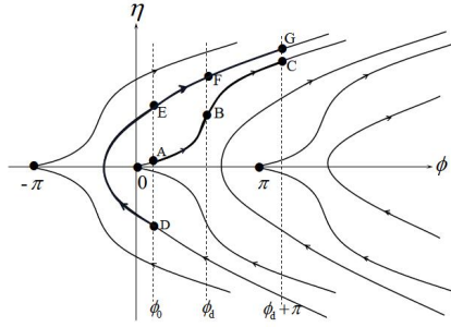
Figure 7: Three types of solutions in Case II with \gamma_2 < 0 for m \geq 0 : arcs AB , EF are two monotone 0-winding solutions and DEF is non-monotone 0-winding solution; arcs ABC , EFG are two monotone 1-winding solutions and DEFG is a non-monotone 1-winding solution.
