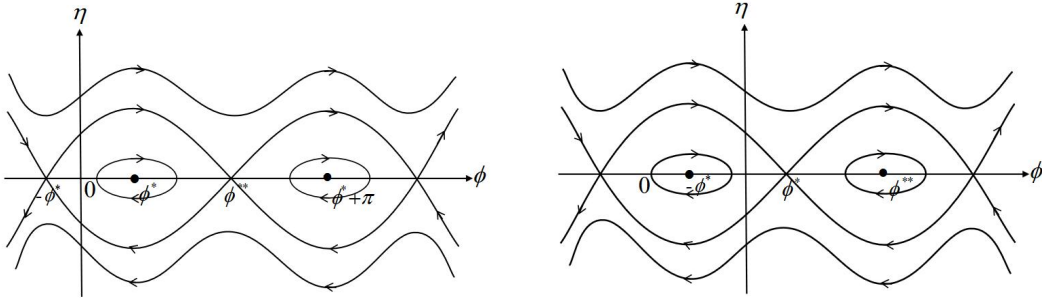
Figure 3: Phase plane portrait for Case III1 where \int_0^\pi \frac{h(t)}{g(t)} dt = 0 . Left panel: -\gamma_2 > \gamma_1 > 0 ; Right panel: \gamma_2 > \gamma_1 > 0 .
