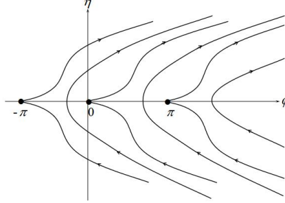
Figure 2: Sketch of the phase plane portrait for Case II with -\gamma_2 = \gamma_1 .
