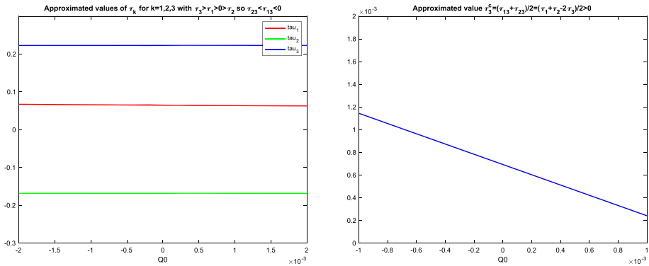
Fig. 7 Numerical examples with L = (0.0001, 0.01, 0.0102) , R = (0.1, 10, 10.2) , and V = 3.4 . Left: \tau_3^c < 0 with \tau_3 > \tau_1 > 0 > \tau_2 , particularly, \tau_{23} < \tau_{13} < 0 for \alpha_1 < \theta_3^c and \alpha_2 < P_3^c(\alpha_1) ; Right: \tau_3^c > 0 for \alpha_1 > \theta_3^c or \alpha_2 > P_3^c(\alpha_1)
