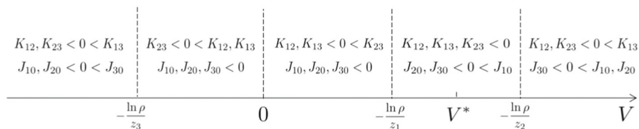
Fig. 6 Signs of K_{ij} and J_{k0} for V \neq V^* and \rho < 1 . Also, as V \rightarrow V^* one always has K_{ij} < 0 in limit, and hence, V_{ij} exists as in the case \sigma_{10} = \sigma_{20}
