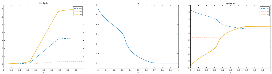
Fig. 3 Profiles of concentrations ( left ), electric potential ( middle ) and electrochemical potentials ( right ) with Q_0 = -.0008 , L = (.01, .001, .021) , R = (10/3, 1/3, 7) , and V = V^* \approx 5.6276
