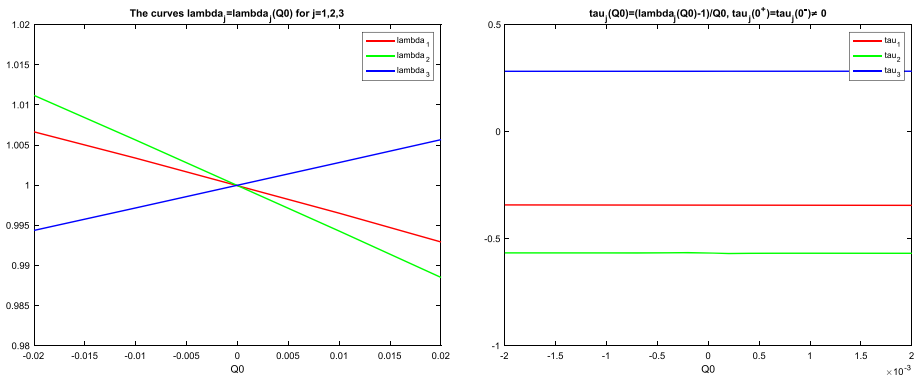
Fig. 4 L = (.01, .001, .021) , R = (10/3, 1/3, 7) , V = V^* \approx 5.6276 : \lambda_j(2Q_0) where \lambda_1(2Q_0) > \lambda_2(2Q_0) for Q_0 > 0 and \lambda_1(2Q_0) < \lambda_2(2Q_0) for Q_0 < 0 (left); \tau_j(0^\pm) \neq 0 and \tau_{12} = \tau_1 - \tau_2 > 0 (case (iii) in Corollary 4.5) (right)
