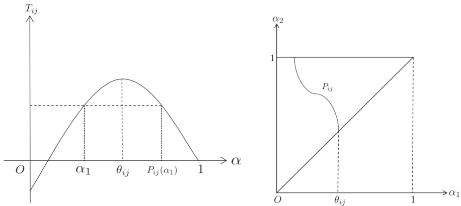
Fig. 1 Function T_{ij} on \alpha and P_{ij} for case (ii) a in Proposition 3.9
