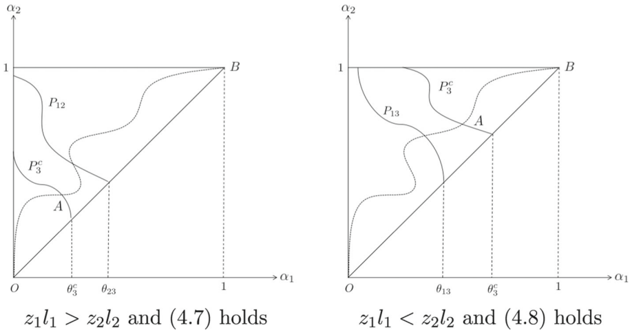
Fig. 5 Graphs of function P_3^c in domain \Delta when V = V^* . Let OB be any curve in \Delta intersecting P_3^c at A . From O to A to B , if z_1 l_1 > z_2 l_2 and (4.7) holds, then \tau_3^c changes from positive to zero to negative; if z_1 l_1 < z_2 l_2 and (4.8) holds, then \tau_3^c changes from negative to zero to positive
