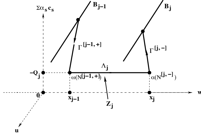
Figure 1: A singular orbit over [x_{j-1}, x_j] projected to the space of variables u , \sum \alpha_s c_s and w : \Gamma^{[j-1,+]} is a singular layer at x = x_{j-1} from B_{j-1} to \mathcal{Z}_j and \Gamma^{[j,-]} from \mathcal{Z}_j to B_j , and \Lambda_j connects “landing” points of \Gamma^{[j-1,+]} in \omega(N^{[j-1,+]} ) and “departing” points of \Gamma^{[j,-]} in \alpha(N^{[j,-]}) on \mathcal{Z}_j .
