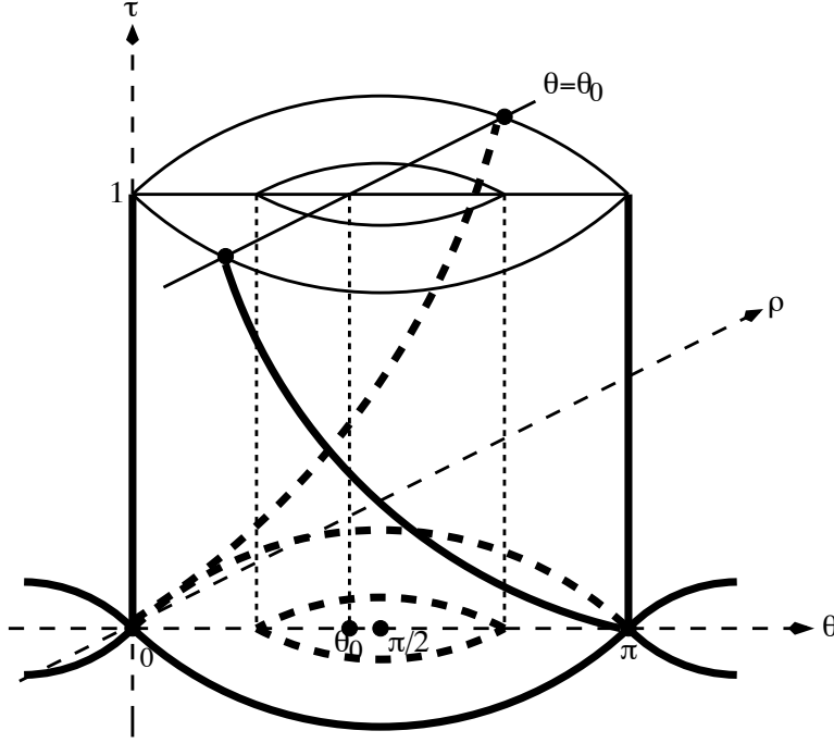
Figure 1: Thick curves are orbits of system (2.16). On \{\tau = 0\} , there are two heteroclinic orbits between (0, 0) and (\pi, 0) ; inside the heteroclinic loop are periodic orbits centered about (\pi/2, 0) . Every cylinder over each orbit on \{\tau = 0\} is invariant. For any \theta_0 \in [0, \pi) , there are two solutions symmetric to each other, one approaches (0, 0, 0) and the other (\pi, 0, 0) as \tau \rightarrow 0 .
